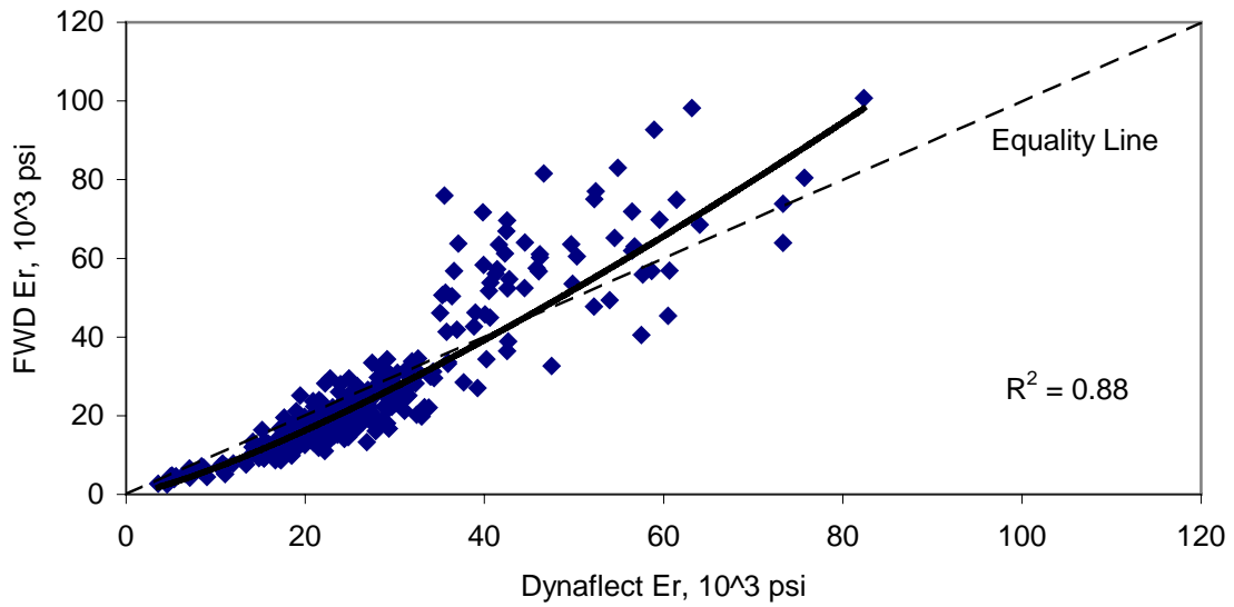
Figure 3 Illustrative comparison of FWD and Dynaflect subgrade moduli
