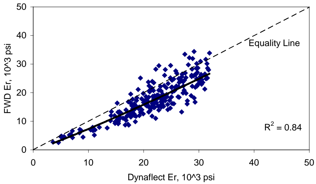
Figure 3 Illustrative comparison of FWD and Dynaflect subgrade moduli
