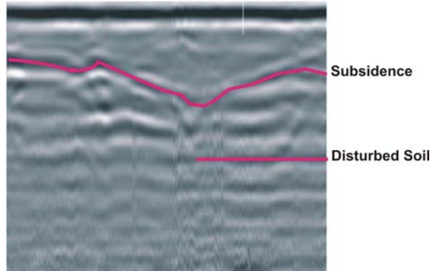
Figure 3: Example GPR Profile Collected at Greenwoods Cemetery exhibiting Subsidence and Disturbed Soil Features
