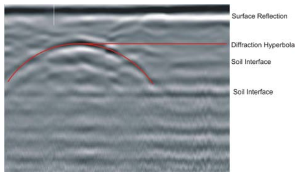
Figure 2: Example GPR Profile Collected at Greenwood Cemetery Exhibiting Hyperbolic Diffraction
